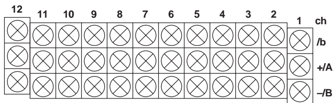
Screw type for DX112P
