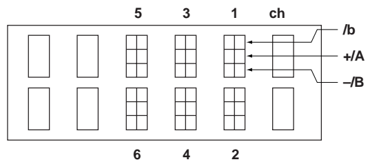
Clamp type for DX112P (/H2)
